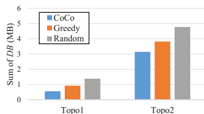
Fig. 7. Sum of Delayed Bytes
